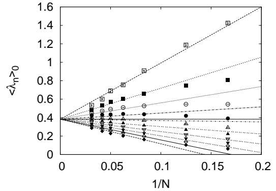
Figure 1: The VEV \langle \lambda_n \rangle_0 with respect to the phase-quenched partition function Z_0 up to N = 32 .
