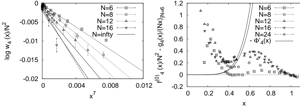
Figure 2: (LEFT) \log w_4(x) against x^7 at small x . (RIGHT) \frac{1}{N^2} f_4^{(0)}(x) - \frac{g_4(x)}{Nx} up to N=24 . Its intersection with -\frac{d}{dx} \Phi_n(x) gives the solution \bar{x}_4 .
