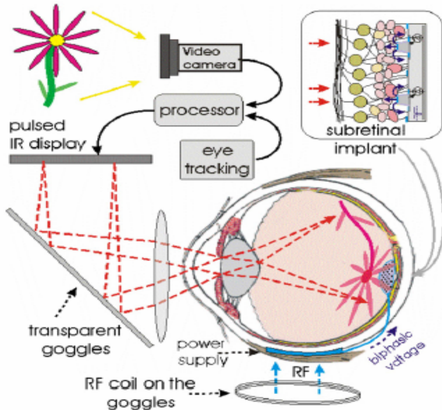
Figure 1. A simplified layout of the general system design including the goggles-mounted video camera, image processor and NIR display. Internally, an extraocular power supply is connected to the subretinal implant. The inset shows a magnified view of a small area of the retinal implant.
